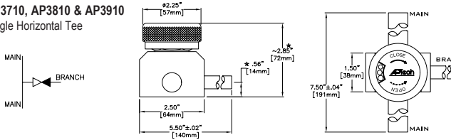
AP3810 shown * VARIES FOR DIFFERENT SIZES OF MAIN
